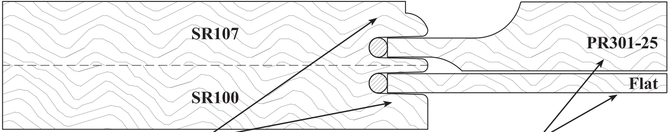
1 3/8" - Full Scale Drawing of a Combination SR107 and SR100 Stile & Rail Profile You may use different Stile & Rail profile for each side of your door.
