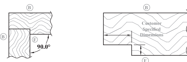
MJ21 90° Inside Corner (Rabbet Option)
