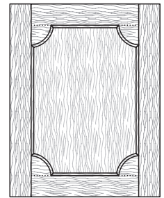
Style: 4080 PC: 211 Frame: PC111 x 0.6 Min. Size: 9¼x9½
