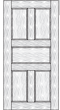
Style: 3465 PC: 236 Frame: PC136 x 0.6 Min. Size: 9¼x16½
