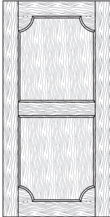
Style: 2419 PC: 228 Frame: PC128 x 0.6 Min. Size: 9¼x12½
