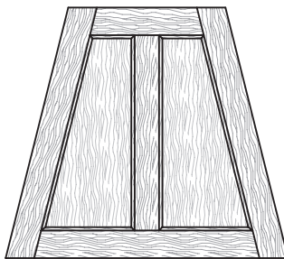
Style: 3235 PC: 226 Frame: PC126 x 0.6 Min. Size: 9¼x8 See Notes for Ordering Information
