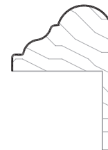
#1206-LF PC: M103 Sq Ft: .72 3/4"W 1 1/32"T
