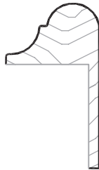
#2094-LF PC: M103 Sq Ft: .82 1 1/16"W 1 7/32"T
