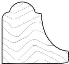
#3044 PC: M103 Sq Ft: .75 1 1/8"W 1 1/32"T
