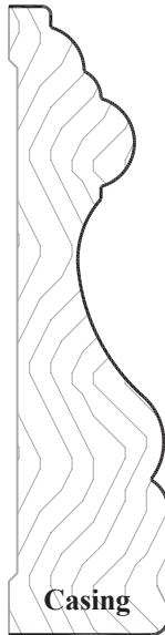
#961 PC: M101 Sq Ft: 1.97 2 1 / 16 "W 3/4"T
