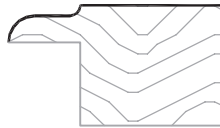
#1021 PC: M101 Sq Ft: .75 1½"W 5/8"T
