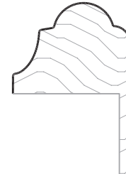
☐ #1277-LF PC: M103 Sq Ft: .72 7/8"W 1 1/32"T
