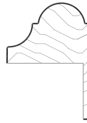
#2471-LF PC: M103 Sq Ft: .80 2 9/32"W 1 1/32"T
