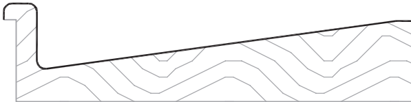
#2276 PC: M101 Sq Ft: 2.06 3 3/2"W 3/4"T
