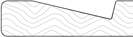
#919 PC: M101 Sq Ft: 1.83 2 3/4"W 3/4"T
