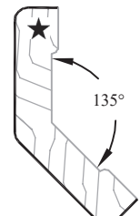
#1279 PC: M101 Sq Ft: .89 2 1/2"W (Inside) 1/4"T
