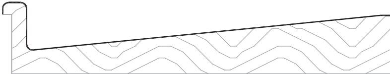
#2276 PC: M101 Sq Ft: 2.06 3 3/2"W 3/4"T
