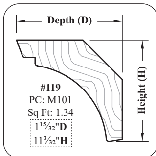
Dimensions (Installed)
