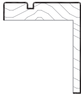
#2931-LF PC: M103 Sq Ft: .72 1 3/16"W 3 1/32"T
