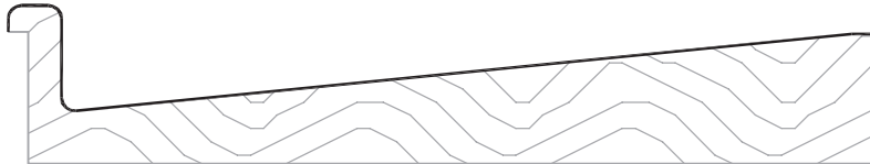
#2276 PC: M101 Sq Ft: 2.06 3\frac{3}{32} "W \frac{3}{4} "T
