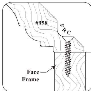
Fastener Relief Cut
