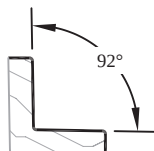
#3142 PC: M101 Sq Ft: .72 1/2"W (Outside) 1/8"T
