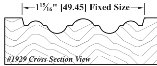
#1929 Cross Section View
