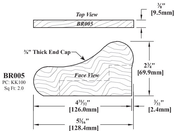
BR005 3/8" Thick End Cap
