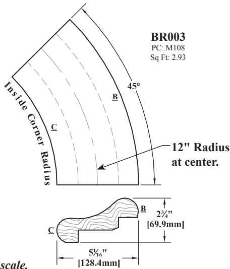
BR003 45° "Inside Corner" Transition Molding
