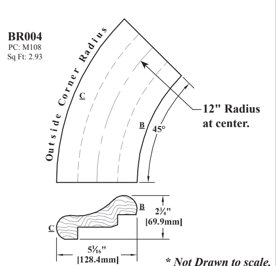
BR004 45° "Outside Corner" Transition Molding
