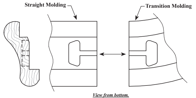
JAM8 Joint Assembly Method - Bolt Lock Rout
