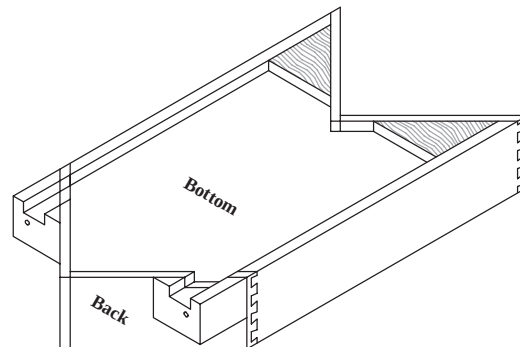
LS102 inside corner drawer box shown with drawer slide blocking DSB200 .
