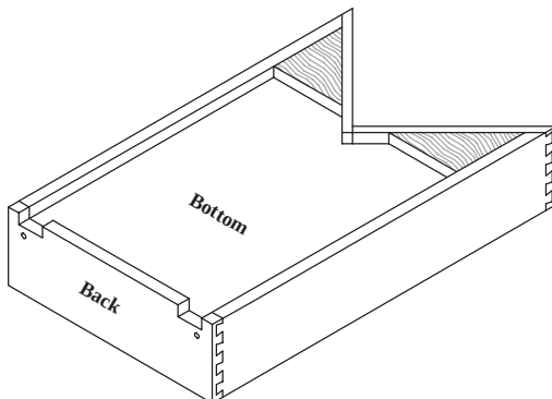
LS101 inside corner drawer box shown with drawer slide blocking DSB100 .
